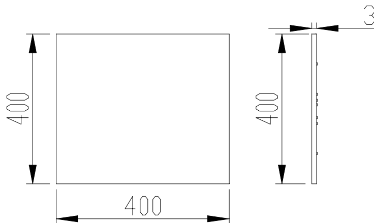
( figure 4 ) Aluminum Radiator Size
